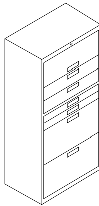
60" H. Case 12" drawer 2x 6" drawers 2x 3" drawers 2x 5" drawers
